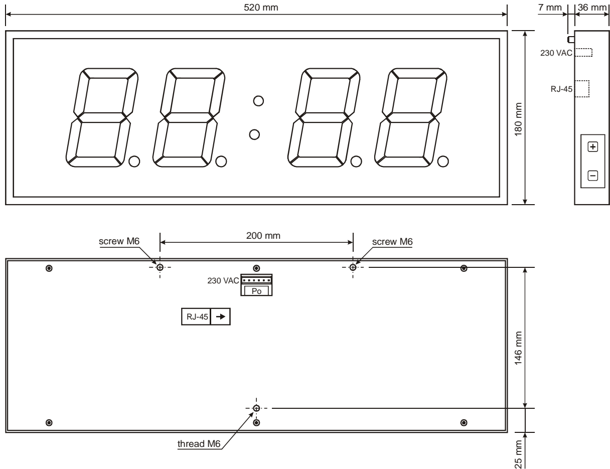
Figure 2: DT100-4R-E drawing (wall mount)
