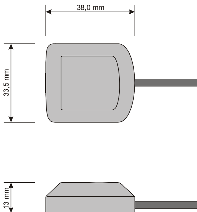
Figure 2: Dimensions of active antenna (MOTOROLA, GC3LP279CA)
